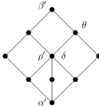
FIGURE 3: I[\alpha', \beta'] .
